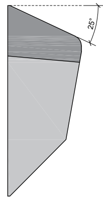
Leaves Short Griffwinke 4
